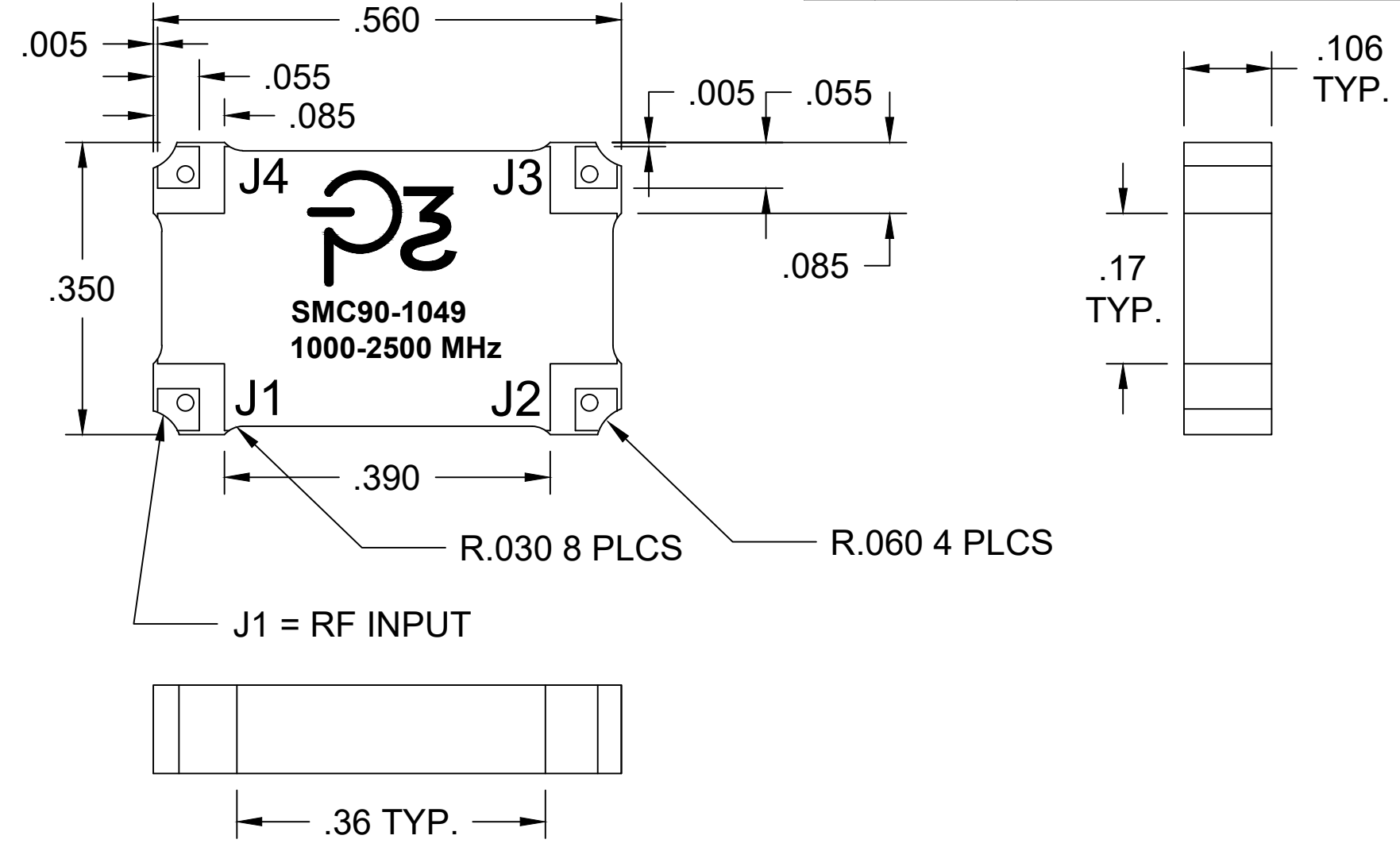
PORT CONFIGURATION
